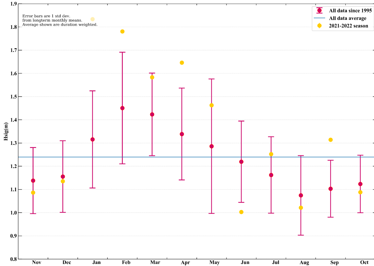
Figure 1. Tweed Heads – Monthly average wave height ( H_s ) for seasonal year and for all data
