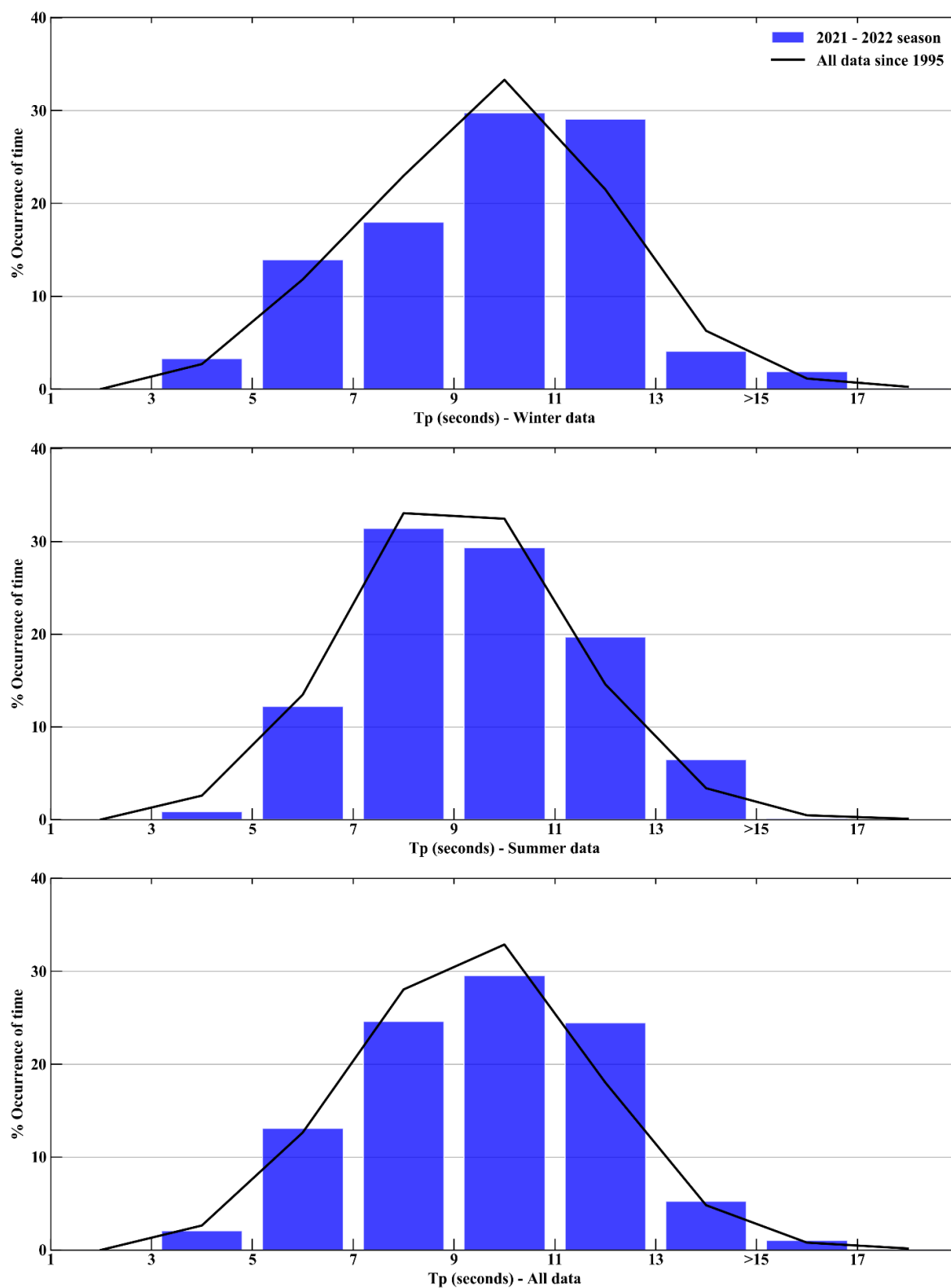
Figure 2. Tweed Heads buoy – histogram percentage (of time) occurrence of wave periods ( T_p ) for all wave heights ( H_s )
