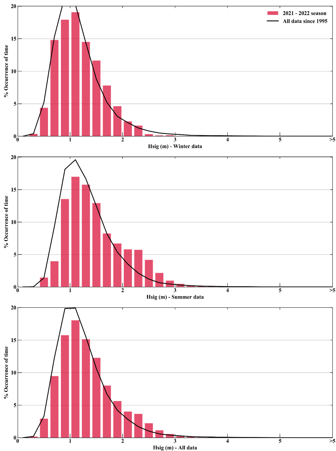
Figure 1. Tweed Heads buoy – histogram percentage (of time) occurrence of wave heights (Hs) for all wave periods (Tp)
