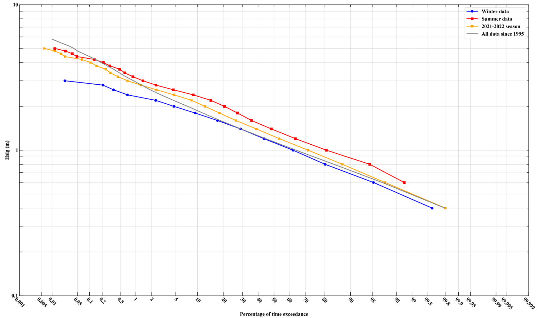
Figure 1. Tweed Heads buoy – percentage (of time) exceedance of wave heights ( H_s ) for all wave periods ( T_p )
